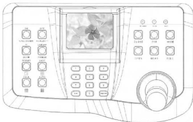
figure 8-1 Image control keyboard panel
