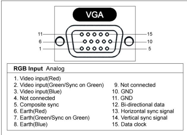
Figure 6 VGA Pin Description
