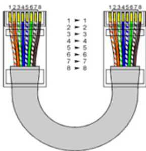
Figure 13 CAT 5 cable color code for EIA/TIA E568B Configuration
