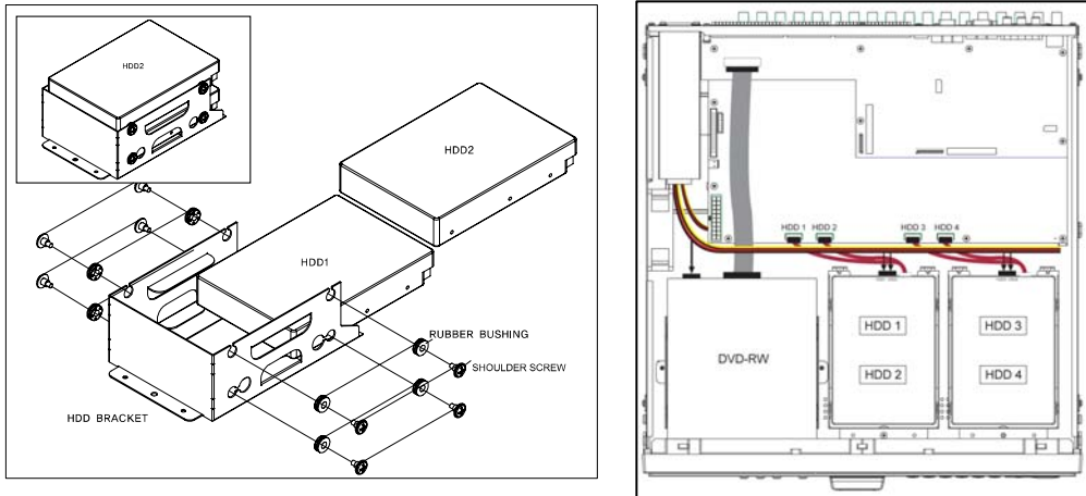
Figure 4 Hard Disk Drive Mounting Bracket
